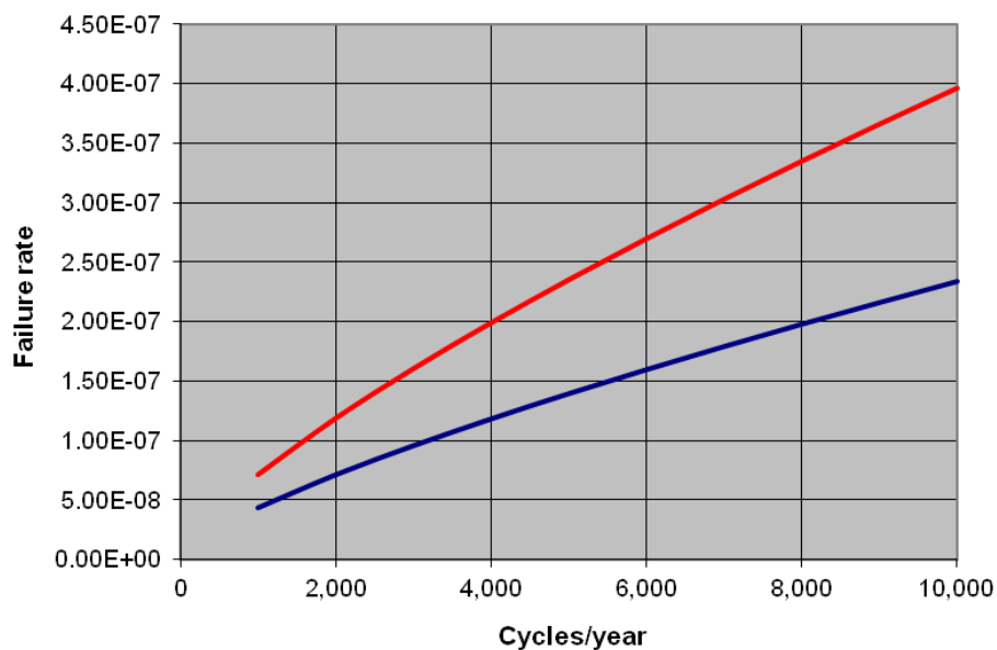
Graph 2: 10/20-series Go Switch 1,000 - 10,000 cycles/year
