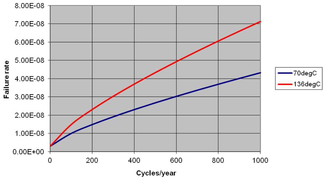
Graph 1: 10/20-series Go Switch 0 - 1,000 cycles/year
