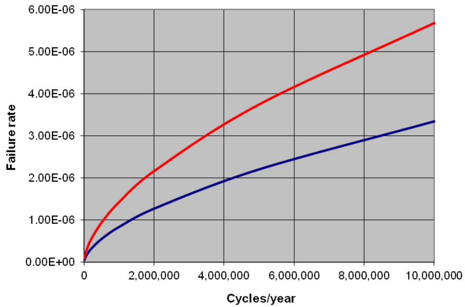
Graph 3: 10/20-series Go Switch >10,000 cycles/year
